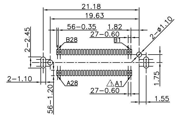
RECOMMENDED 1C PCB LAYOUT
