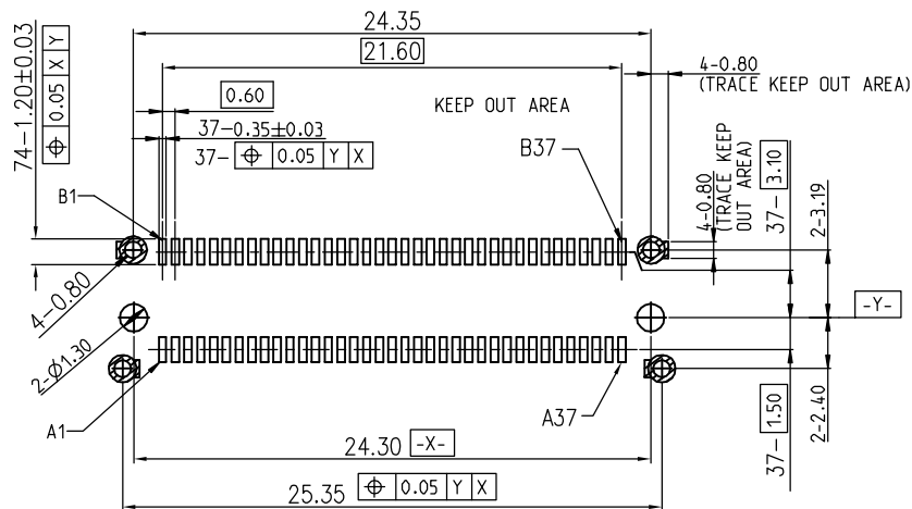
RECOMMENDED PCB LAYOUT (GENERAL TOLERANCES :+/-0.05)
