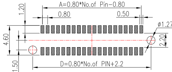
RECOMMENDED PCB LAYOUT(TOP SIDE) PCB BOARD TOLFRANCF±0.05
