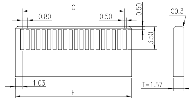
ROMMENED PLUG-PCB LAYOUT TOLERANCE ±0.05
