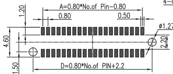
RECOMMENDED PCB LAYOUT(TOP SIDE) PCB BOARD TOLFRANCE±0.05
