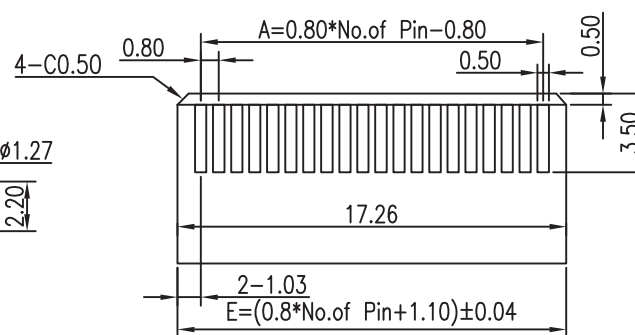
ROMMENDED PLUG-PCB LAYOUT TOLERANCE ±0.05
